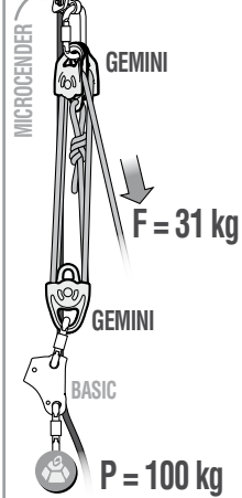
6D. 4:1 hauling system with progress capture for double pulleys
