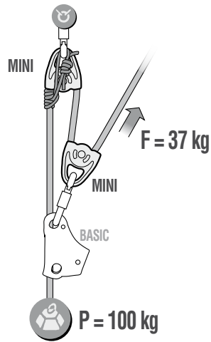
6C. 3:1 hauling system
